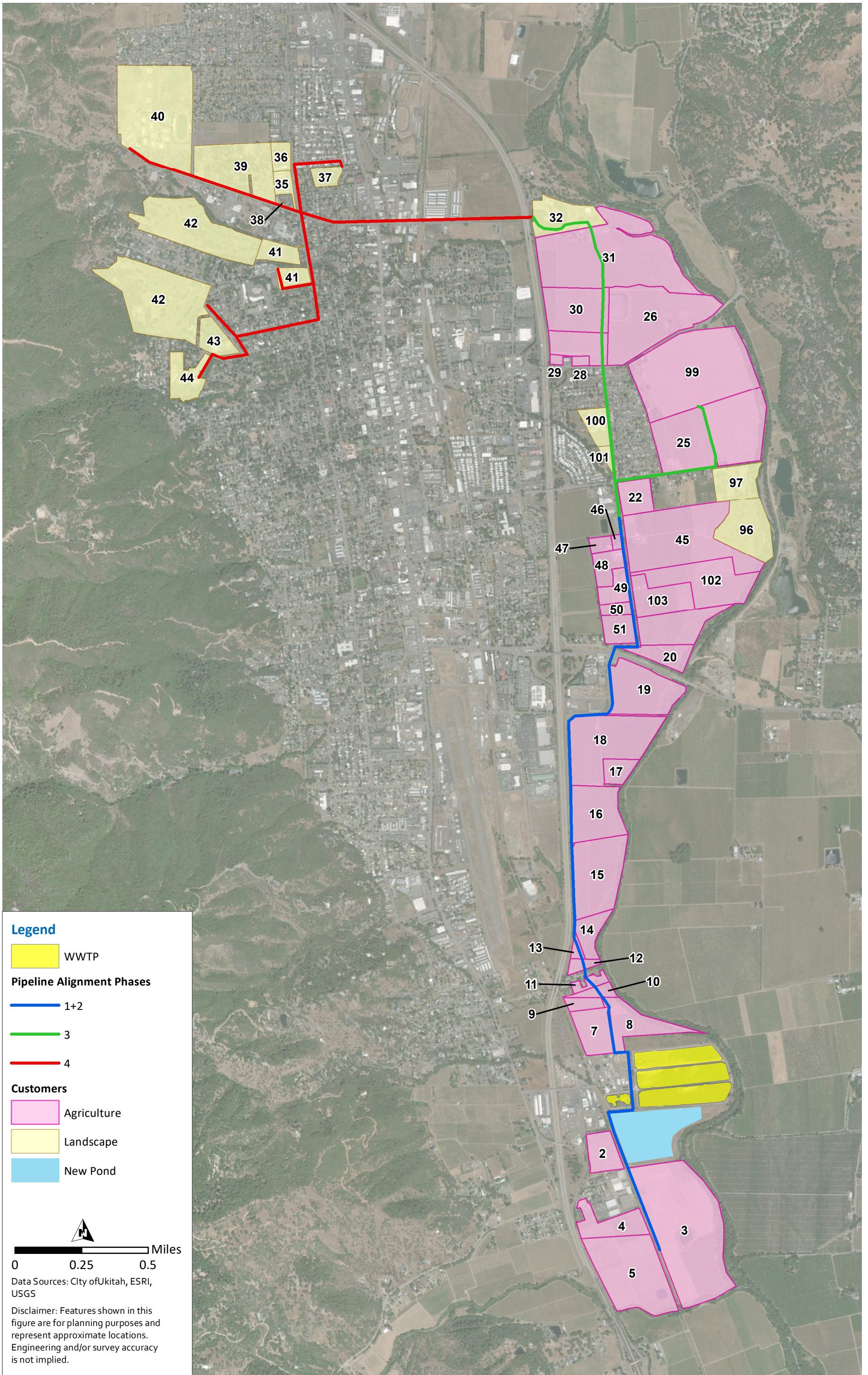
Figure 1 Phase 1 - Phase 4 Pipe Alignment
